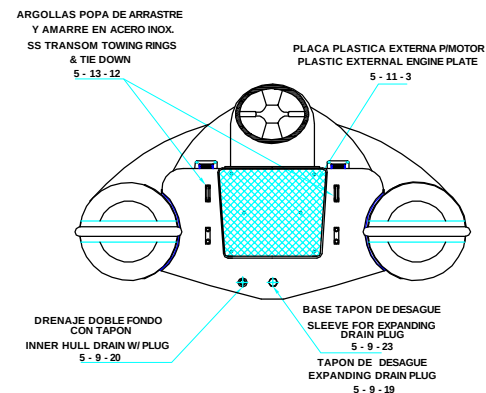
AFT VIEW VISTA TRASERA
